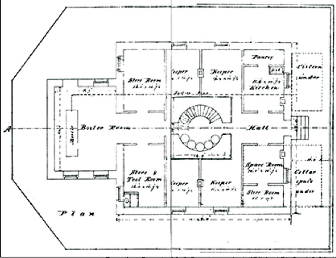
Douglas County Mail Courtesy photo/Gibbs/ Binford & Mort The original floorplan for the lighthouse as originally constructed. Note the absence of indoor plumbing facilities; calls of Nature were answered in a tiny outhouse that hung directly over the ocean at the edge of the bluff.
